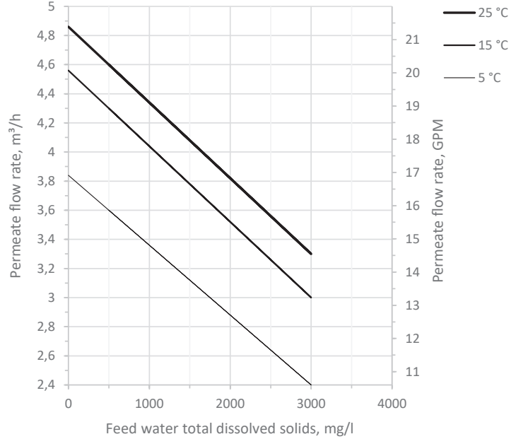
ECOSOFT MO3 RO FLOW CAPACITY GRAPH (WITH XLE-440 MEMBRANES)
